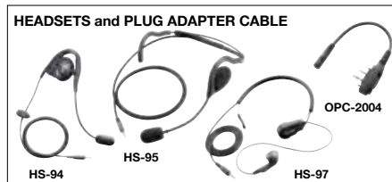
HS-94 : Earhook headset with flexible boom microphone. HS-95 : Behind-the-head headset with flexible boom microphone. HS-97 : Throat microphone that fits around your neck and picks up speech vibrations. OPC-2004 : Required when using any of these headsets.
